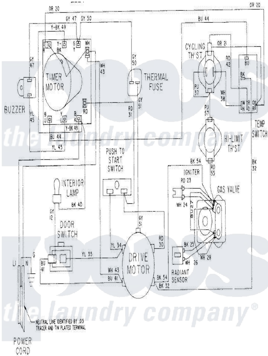
Maytag Residential Maytag LDG4914AAL Dryer Parts Parts Diagram 08 - WIRING INFORMATION-LDG4914 Click on the part number to view part
