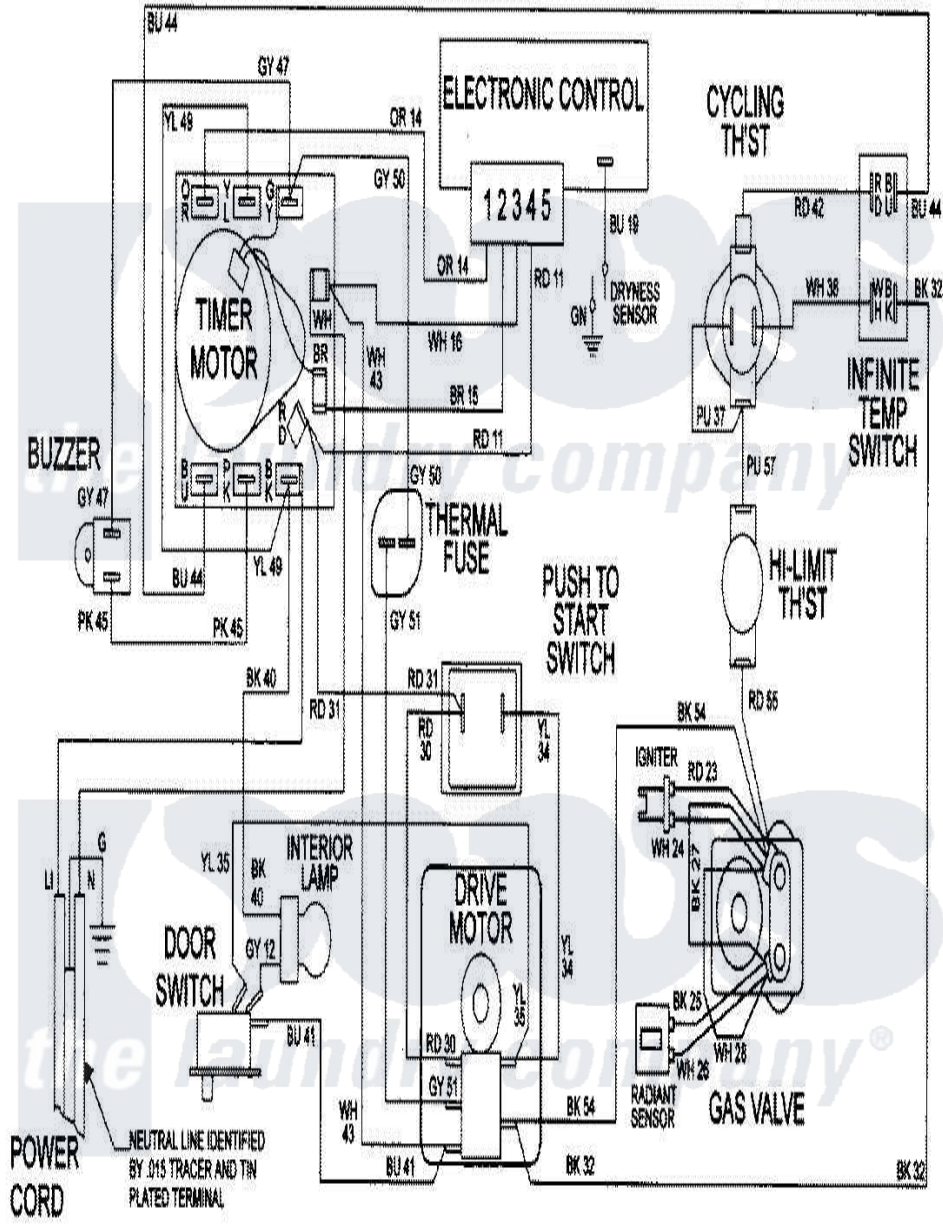
Maytag Residential Maytag LDG5916AAM Dryer Parts Parts Diagram 09 - WIRING INFORMATION Click on the part number to view part
