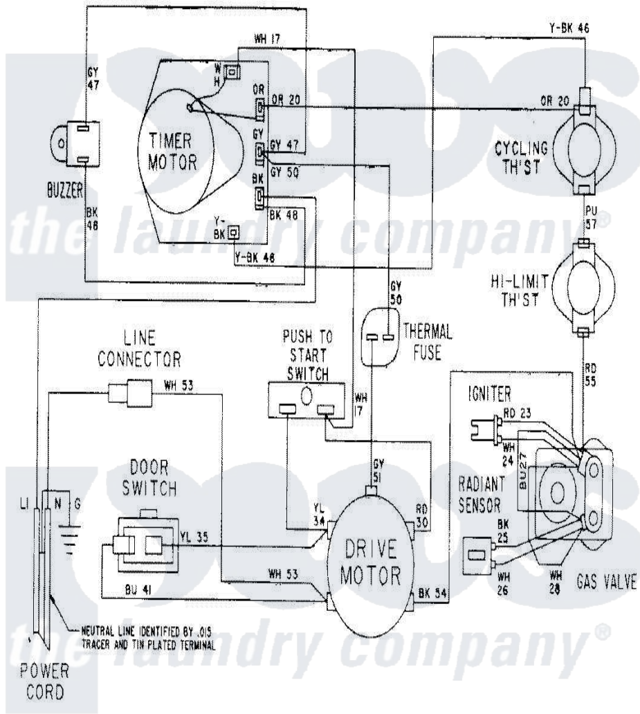
Maytag Residential Maytag LDG6004AAW Dryer Parts Parts Diagram 09 - WIRING INFORMATION-LDG6004AAW
