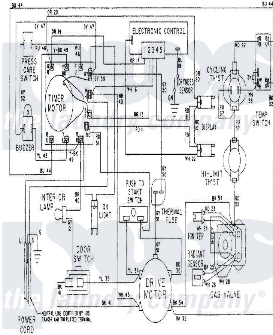
Maytag Residential Maytag LDG6914AAM Dryer Parts Parts Diagram 09 - WIRING INFORMATION-LDG6914 Click on the part number to view part
