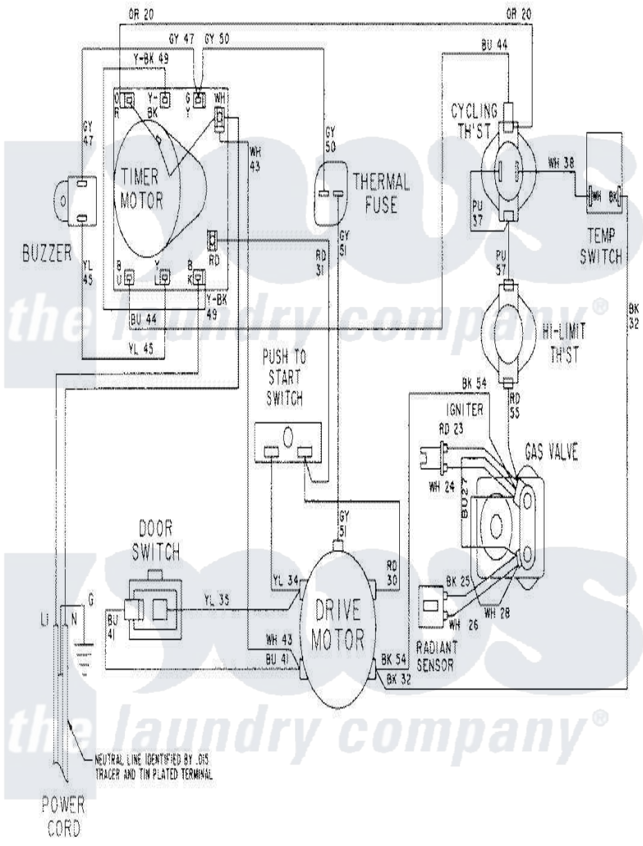
Maytag Residential Maytag LDG8304AAL Dryer Parts Parts Diagram 08 - WIRING INFORMATION-LDG8334AAx Click on the part number to view part
