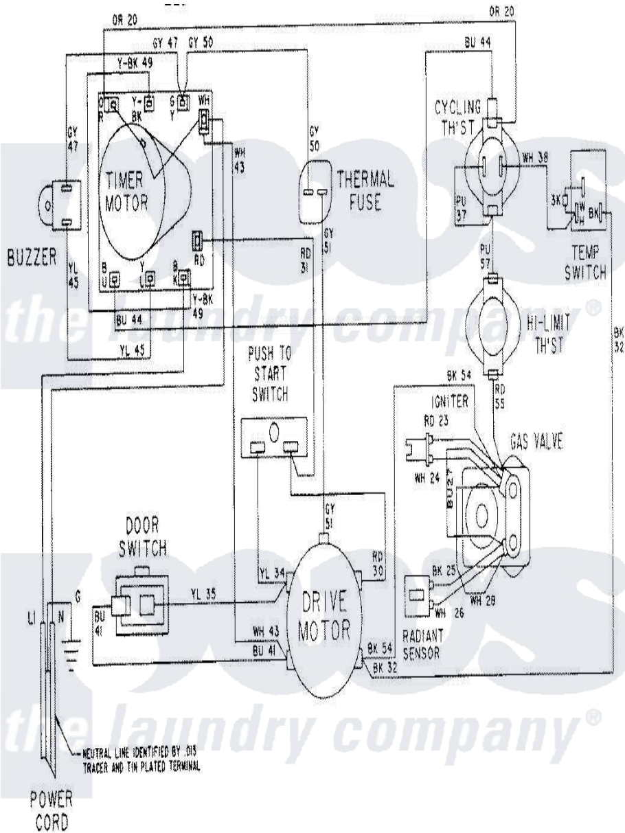
Maytag Residential Maytag LDG8414AAE Dryer Parts Parts Diagram 08 - WIRING INFORMATION-LDG8414AAx Click on the part number to view part
