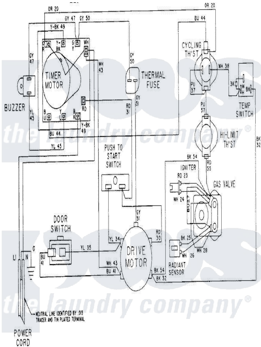
Maytag Residential Maytag LDG8414AAL Dryer Parts Parts Diagram 08 - WIRING INFORMATION-LDG8414AAx Click on the part number to view part
