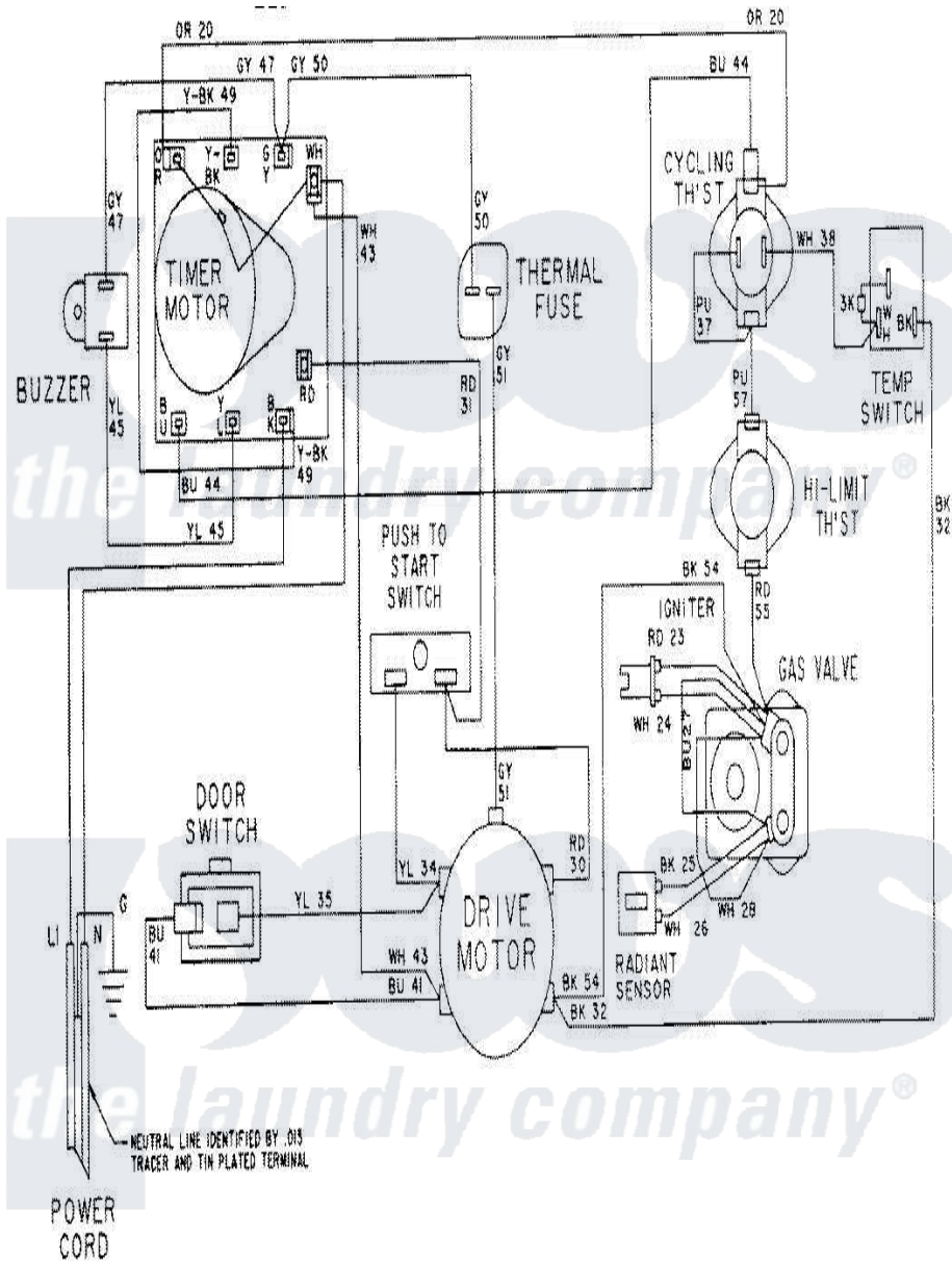
Maytag Residential Maytag LDG8414AAM Dryer Parts Parts Diagram 10 - WIRING INFORMATION-LDG8414AAx Click on the part number to view part
