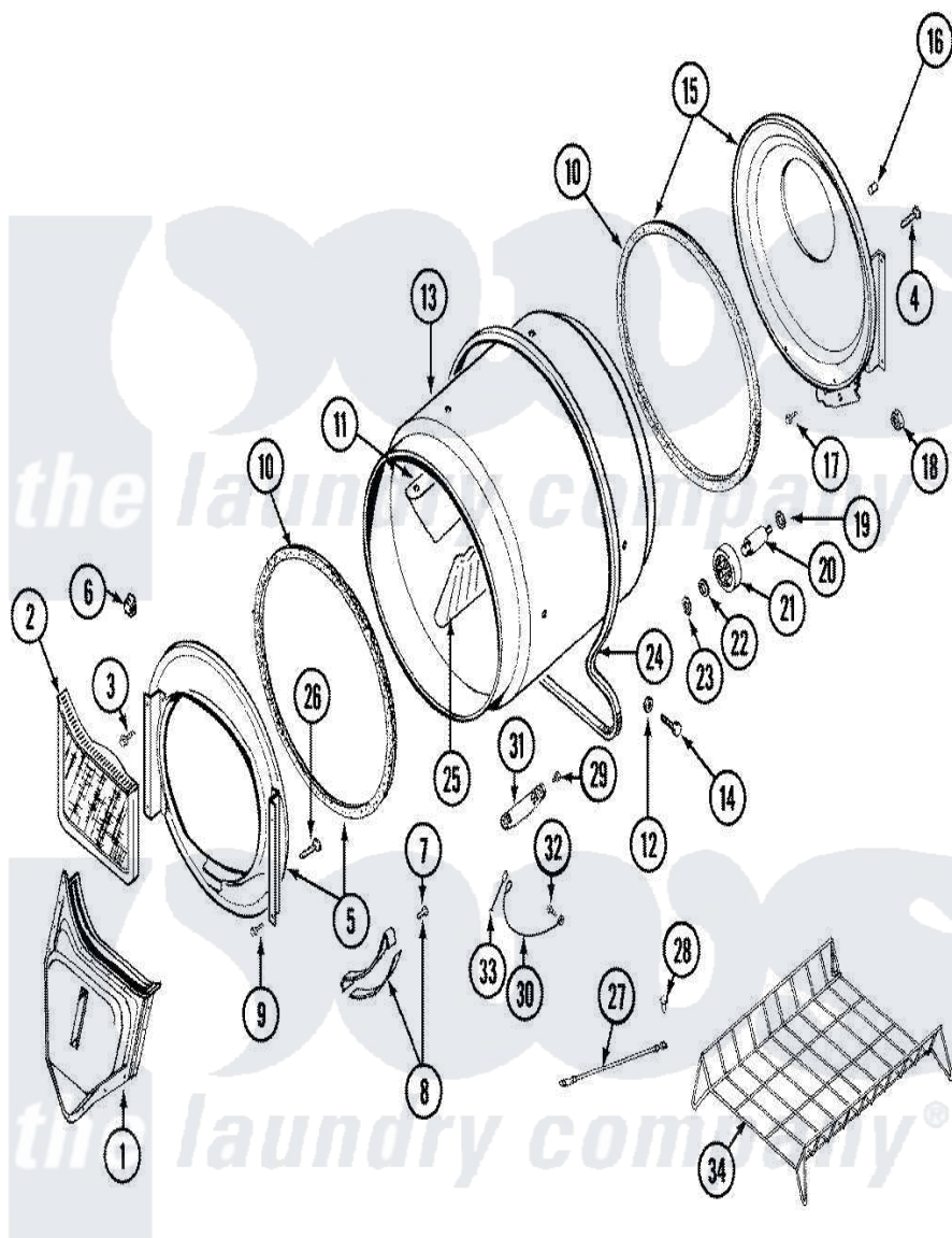
Maytag Residential Maytag LDG8426EGE Dryer Parts Parts Diagram 07 - TUMBLER
