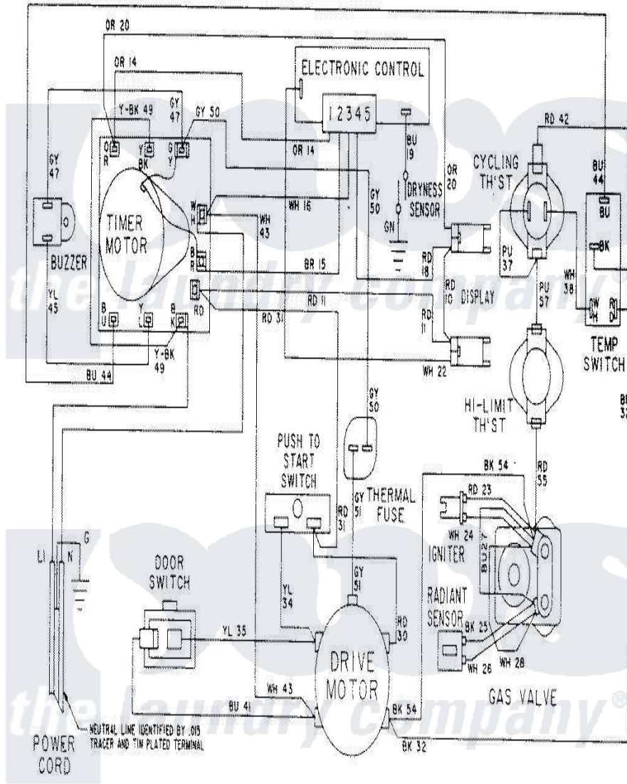
Maytag Residential Maytag LDG8604AAE Dryer Parts Parts Diagram 08 - WIRING INFORMATION-LDG8604AAx Click on the part number to view part
