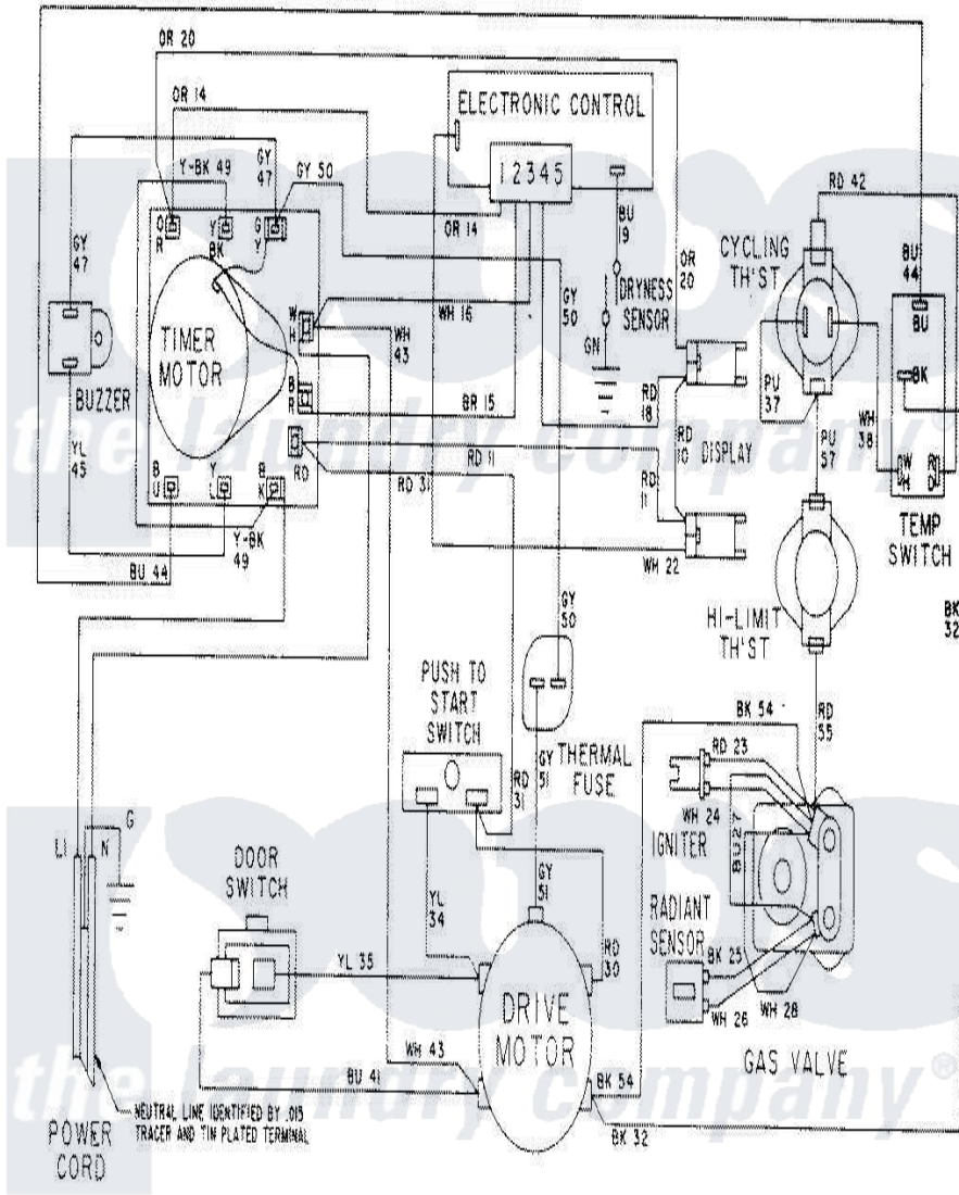
Maytag Residential Maytag LDG8604AAM Dryer Parts Parts Diagram 09 - WIRING INFORMATION-LDG8604AAx Click on the part number to view part
