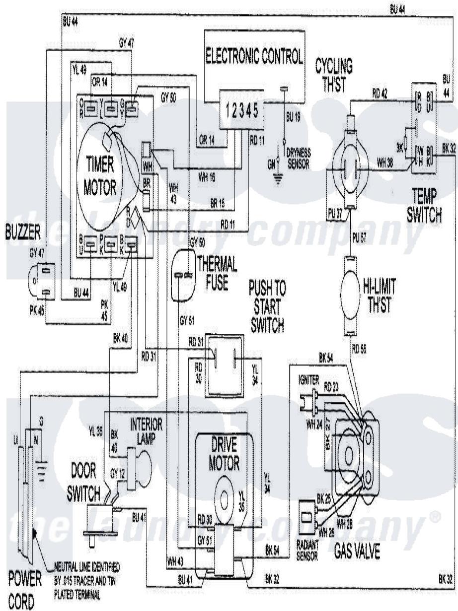
Maytag Residential Maytag LDG8706AAM Dryer Parts Parts Diagram 09 - WIRING INFORMATION Click on the part number to view part
