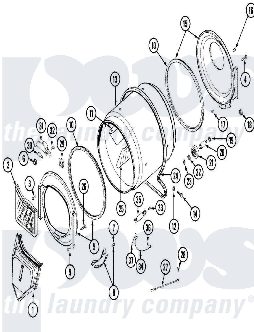
Maytag Residential Maytag LDG8824AAL Dryer Parts Parts Diagram 07 - TUMBLER Click on the part number to view part
