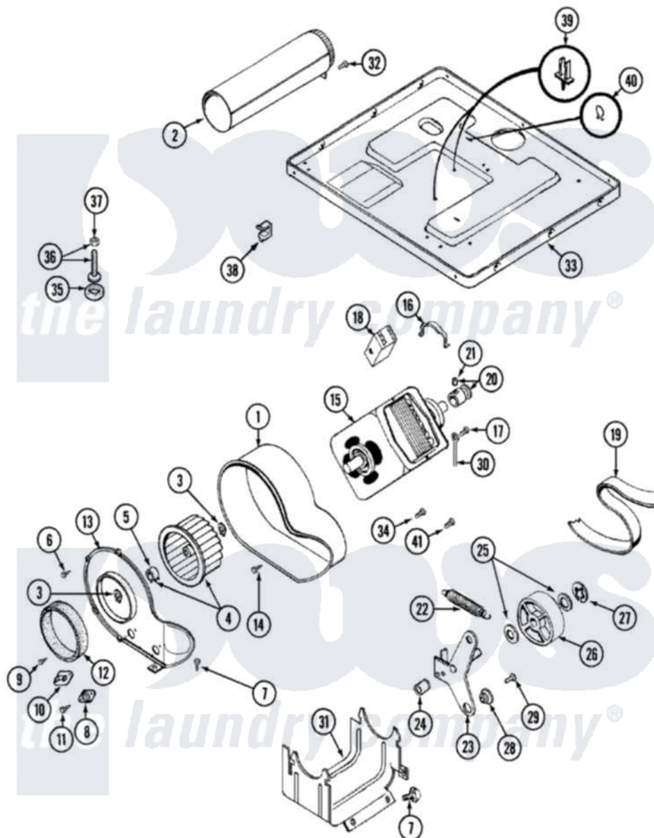
Maytag Residential Maytag LDG9206ABE Dryer Parts Parts Diagram 07 - MOTOR DRIVE Click on the part number to view part
