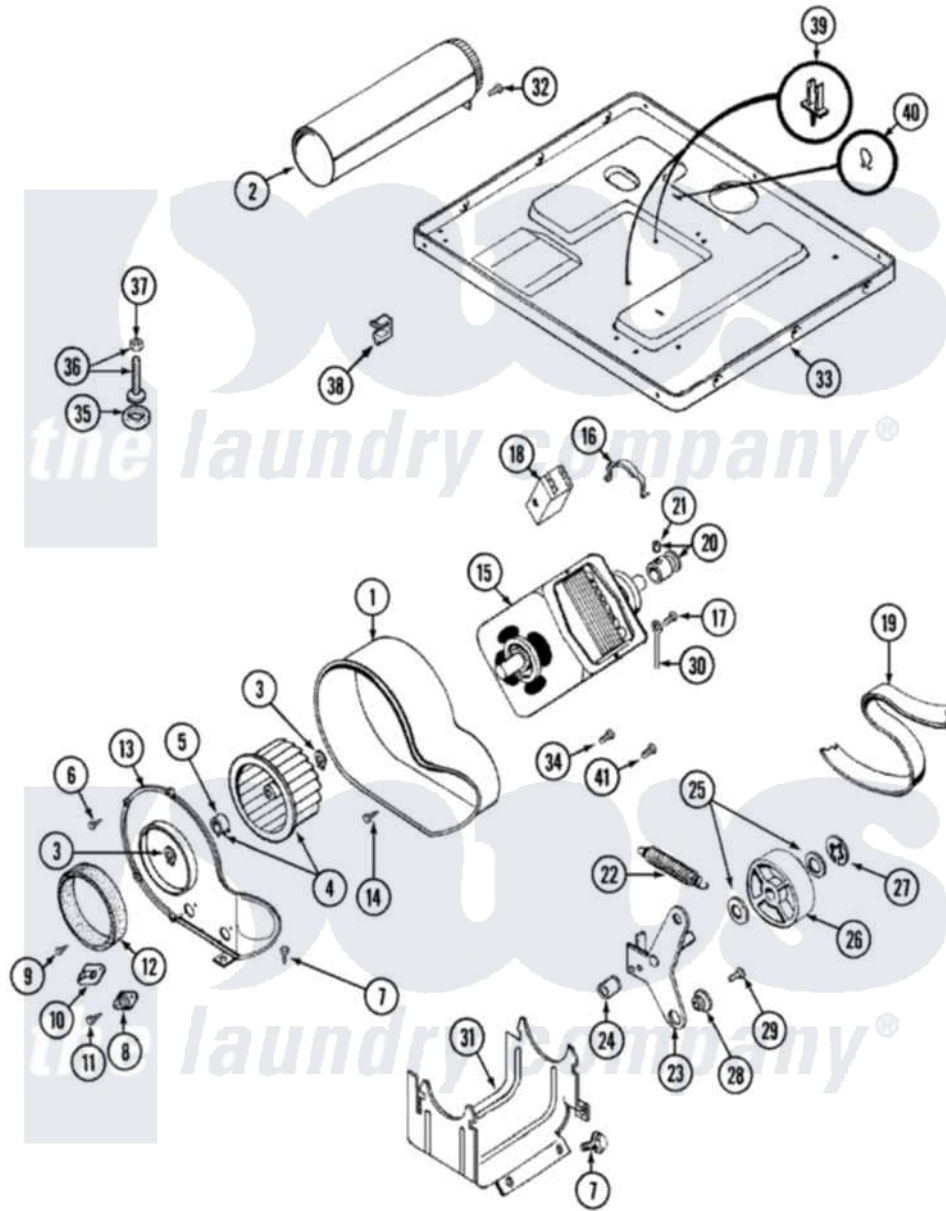
Maytag Residential Maytag LDG9306ABE Dryer Parts Parts Diagram 07 - MOTOR DRIVE Click on the part number to view part
