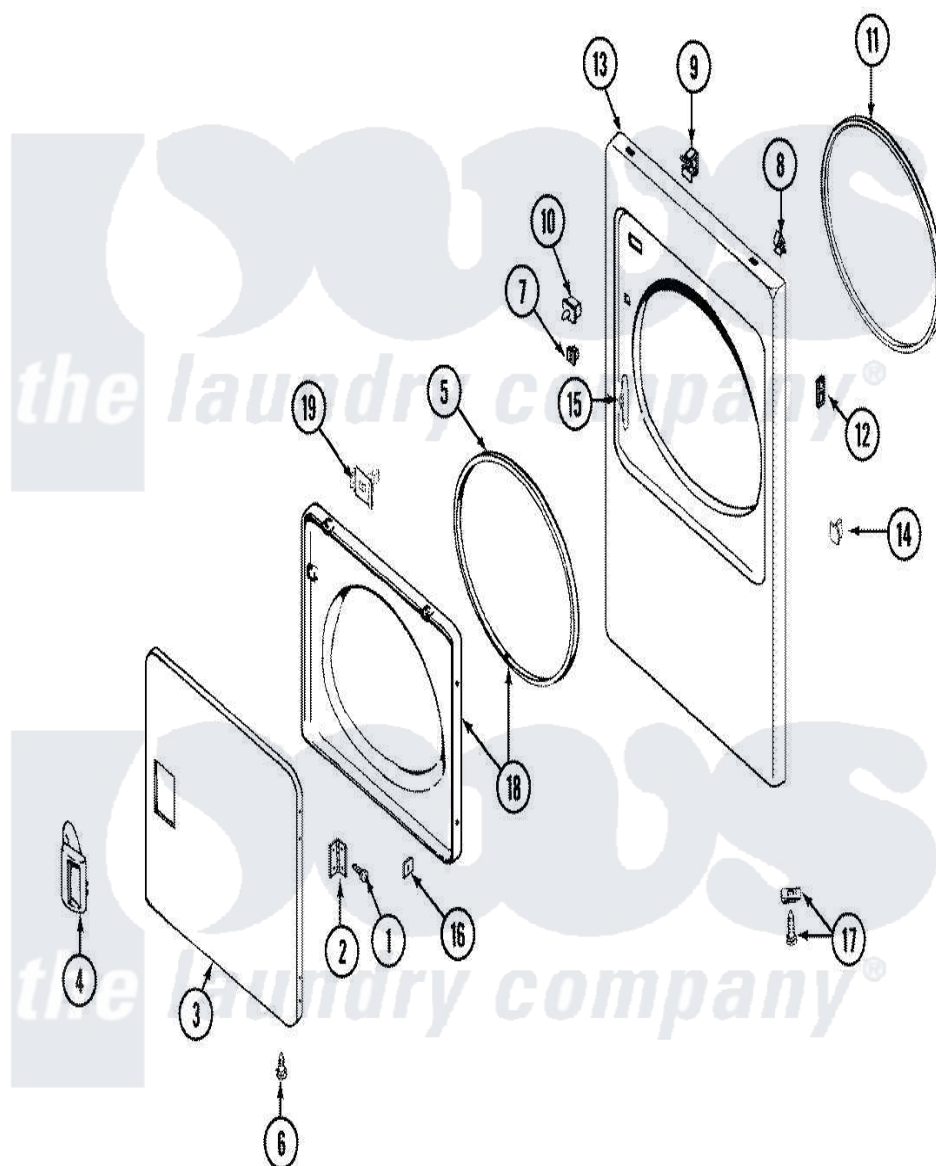
Maytag Residential Maytag LDG9606AAM Dryer Parts Parts Diagram 04 - DOOR Click on the part number to view part
