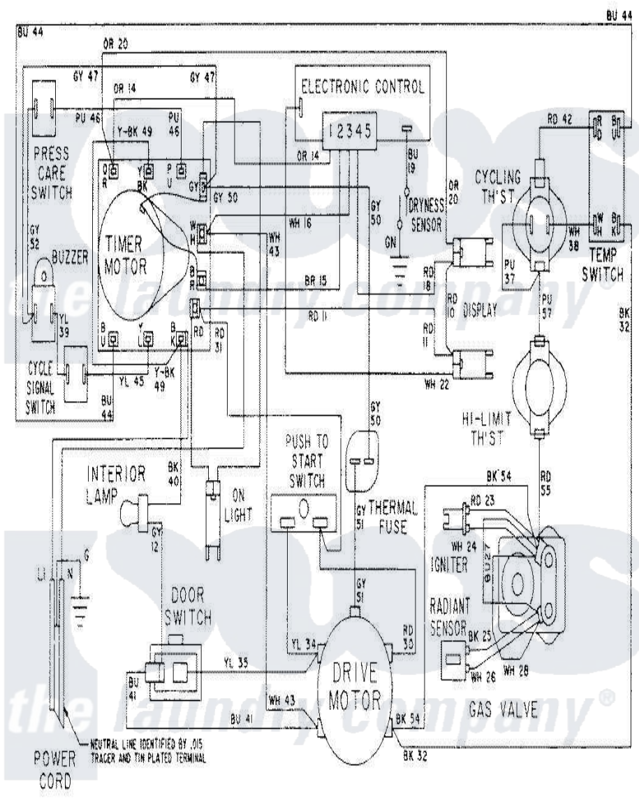
Maytag Residential Maytag LDG9804AAL Dryer Parts Parts Diagram 09 - WIRING INFORMATION-LDG9804AAx Click on the part number to view part
