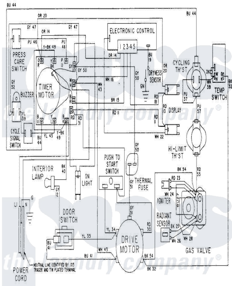
Maytag Residential Maytag LDG9814AAE Dryer Parts Parts Diagram 09 - WIRING INFORMATION-LDG9814AAx Click on the part number to view part
