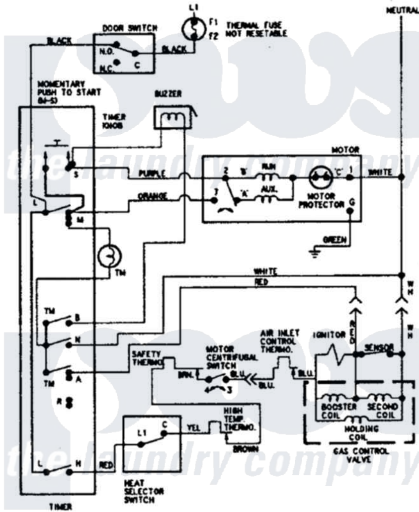
Maytag Residential Maytag LNC8760A71 Dryer Parts Parts Diagram 08 - WIRING INFORMATION Click on the part number to view part
