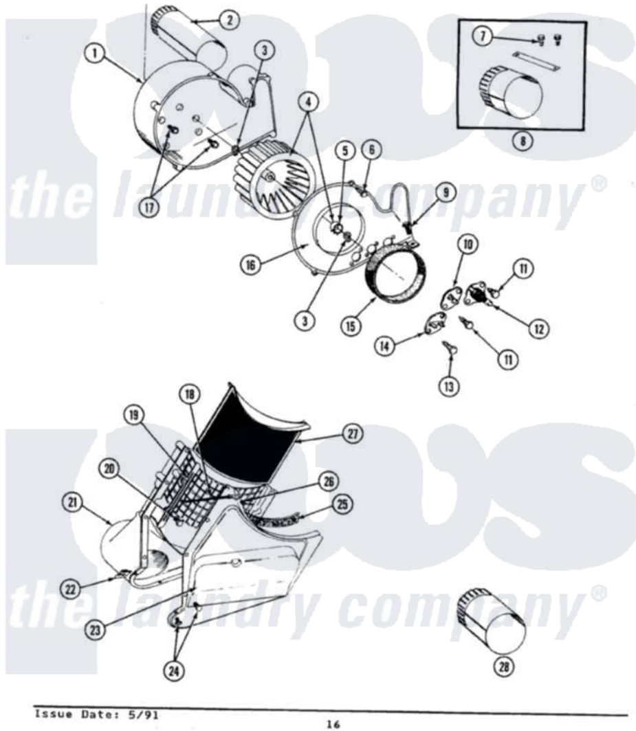
Maytag Residential Maytag LSG1000 Stacked Washer and Dryer Parts Parts Diagram 02 - BLOWER HOUSING/THERMOSTATS & LINT SCREEN Click on the part number to view part
