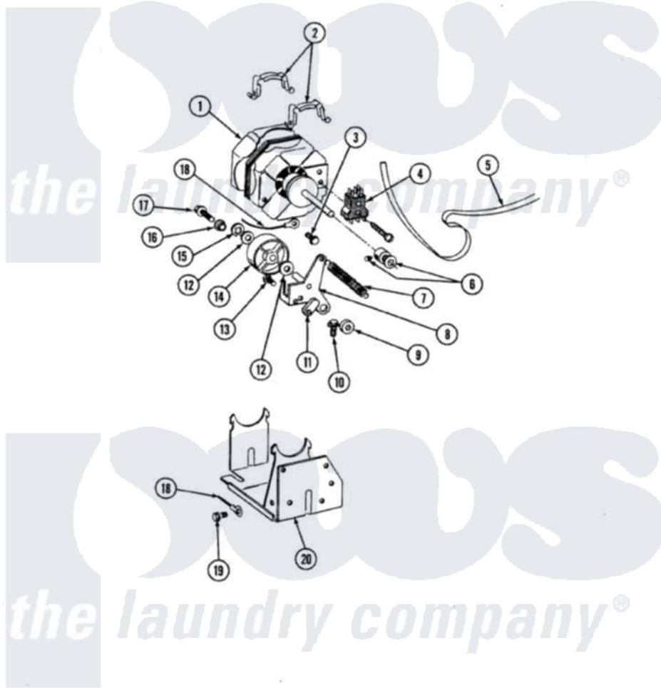
Maytag Residential Maytag LSG1000 Stacked Washer and Dryer Parts Parts Diagram 14 - MOTOR & IDLER ASSEMBLY
