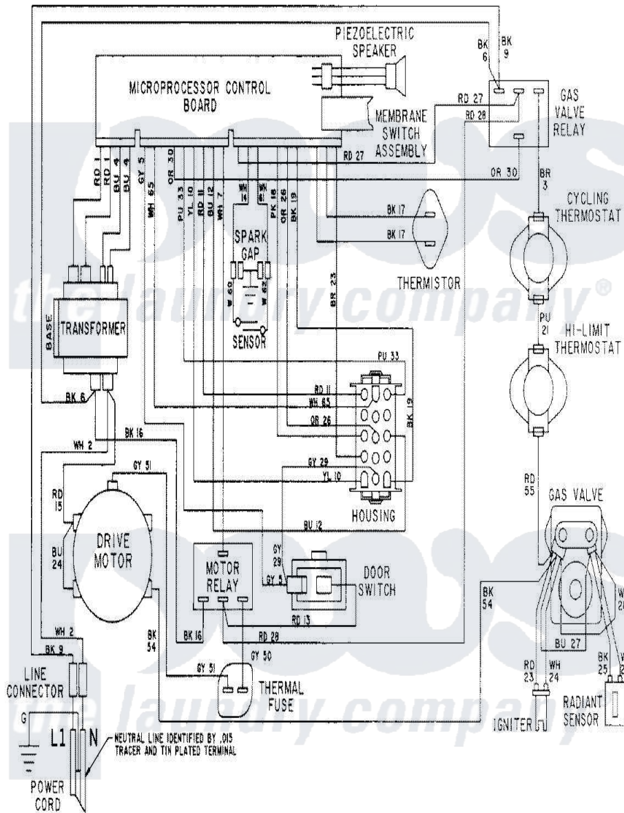
Maytag Residential Maytag LSG9904AAM Stacked Washer and Dryer Parts Diagram 15 - WIRING INFORMATION-LSG9904AAx (DRYER) Click on the part number to view part
