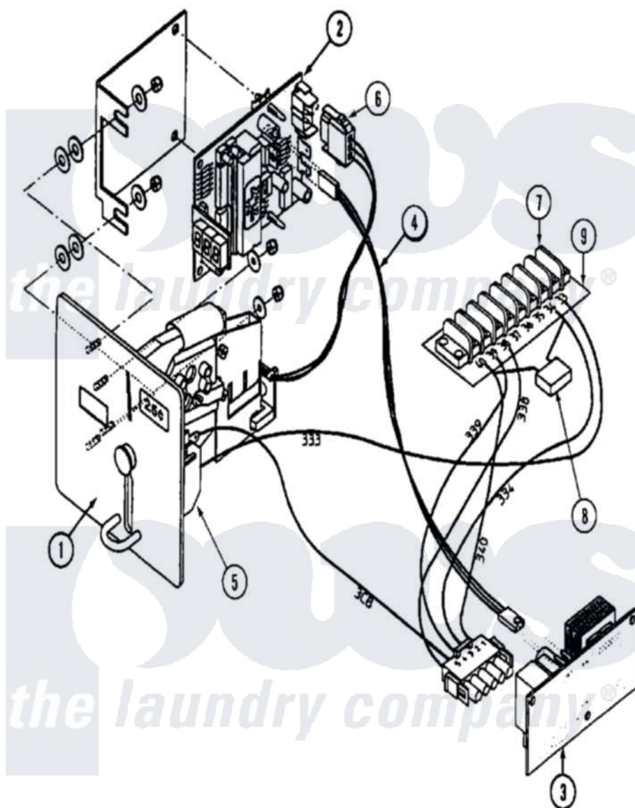
Maytag Residential Maytag MAF18MC4VL Washer Parts Parts Diagram 08 - COIN METER (MAF18MC4Vx) Click on the part number to view part
