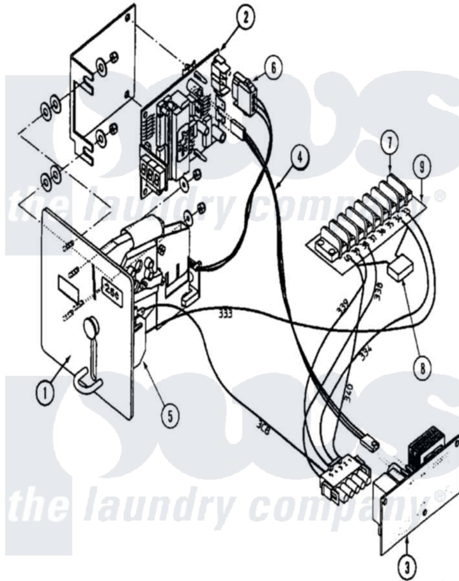
Maytag Residential Maytag MAF25MC4VW Washer Parts Parts Diagram 02 - COIN METER (MAF25MC4Vx) Click on the part number to view part
