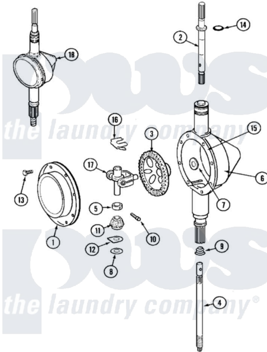
Maytag Residential Maytag MAT10DAAAL Washer Parts Parts Diagram 07 - TRANSMISSION Click on the part number to view part
