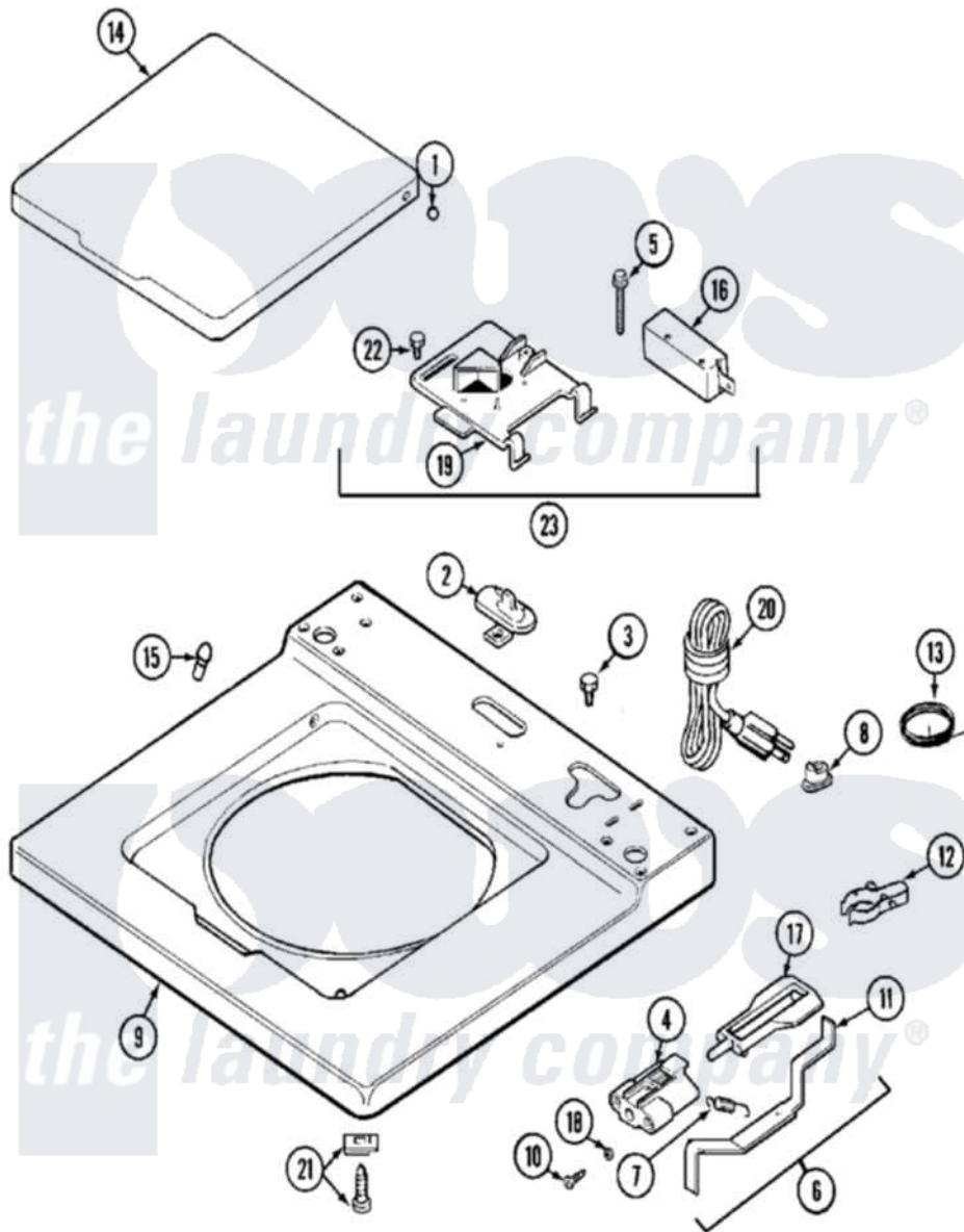
Maytag Residential Maytag MAT10DAABL Washer Parts Parts Diagram 03 - TOP Click on the part number to view part
