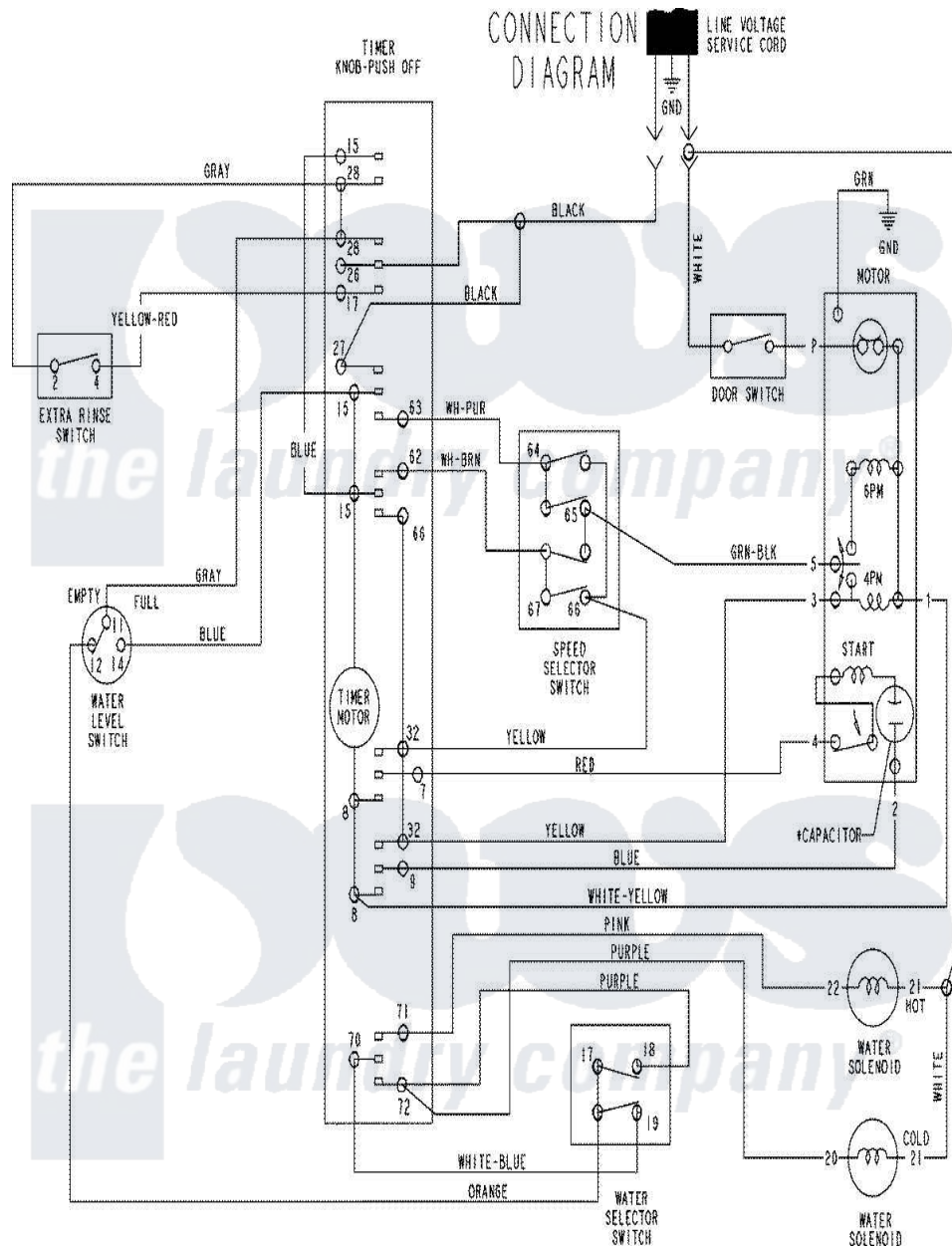
Maytag Residential Maytag MAV2755AJW Washer Parts Parts Diagram 07 - WIRING INFORMATION Click on the part number to view part
