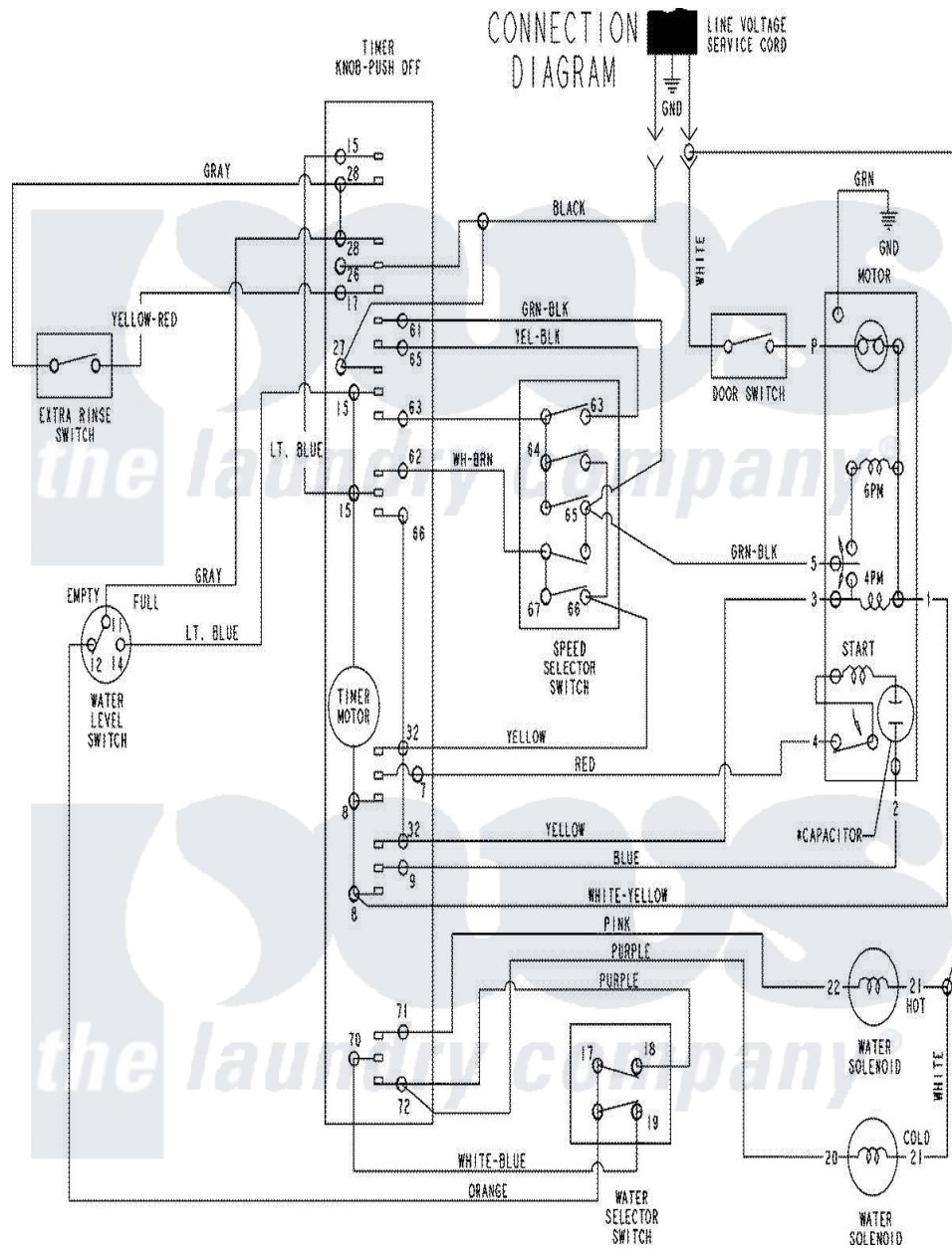
Maytag Residential Maytag MAV275SAWW Washer Parts Parts Diagram 07 - WIRING INFORMATON Click on the part number to view part
