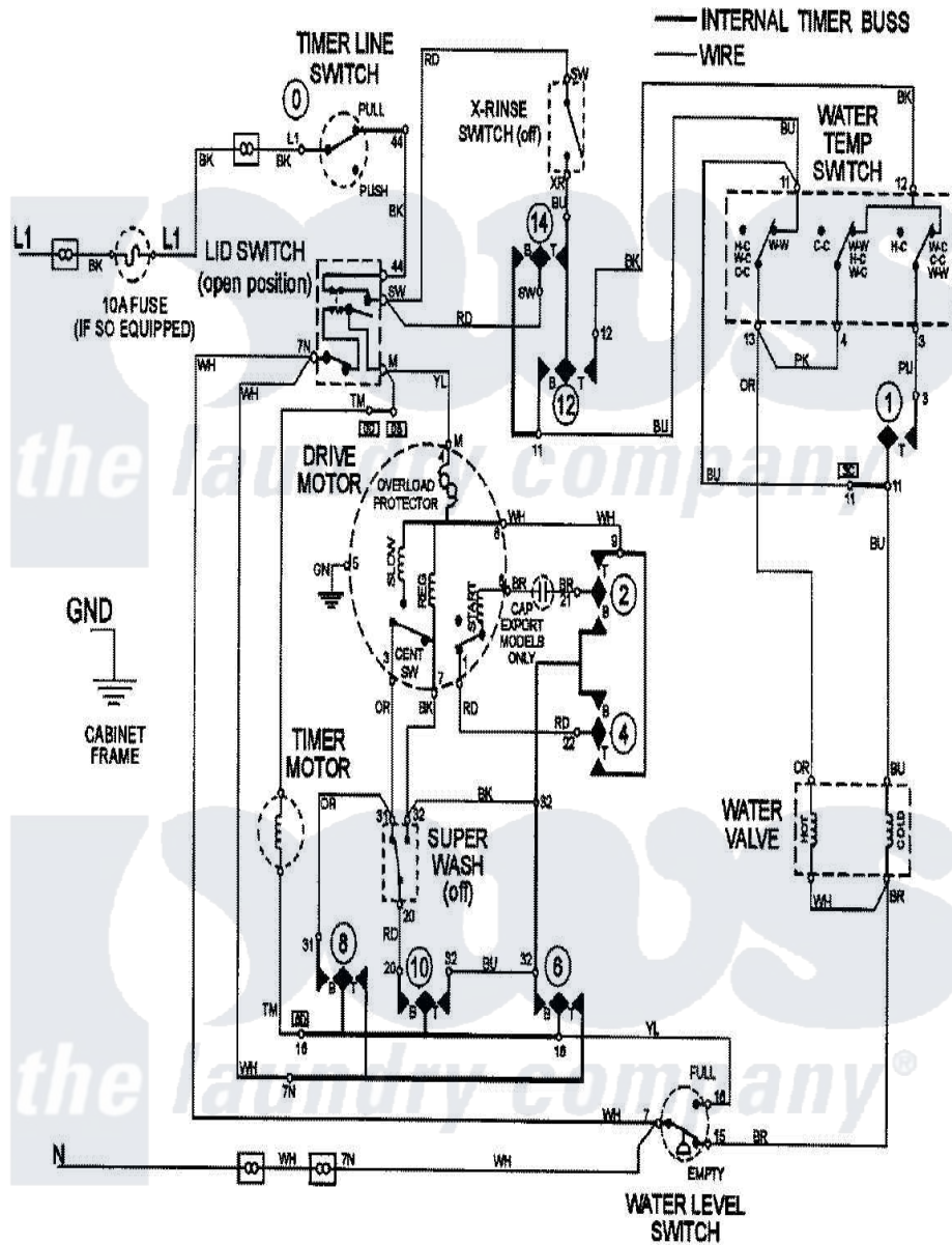
Maytag Residential Maytag MAV5960AWW Washer Parts Parts Diagram 08 - WIRING INFORMATION Click on the part number to view part
