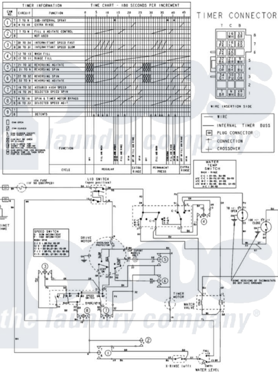
Maytag Residential Maytag MAV6458AWW Washer Parts Parts Diagram 09 - WIRING INFORMATION Click on the part number to view part
