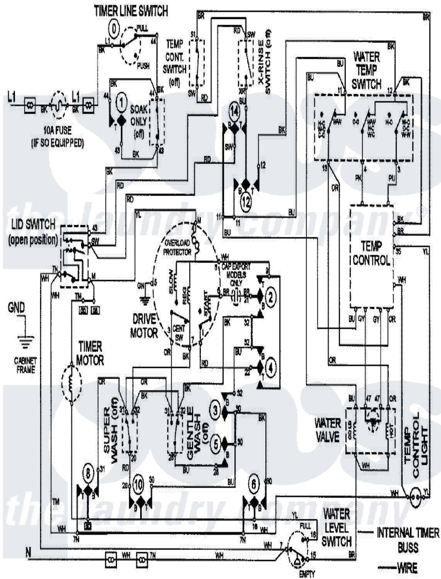
Maytag Residential Maytag MAV7057AWW Washer Parts Parts Diagram 07 - WIRING INFORMATION Click on the part number to view part
