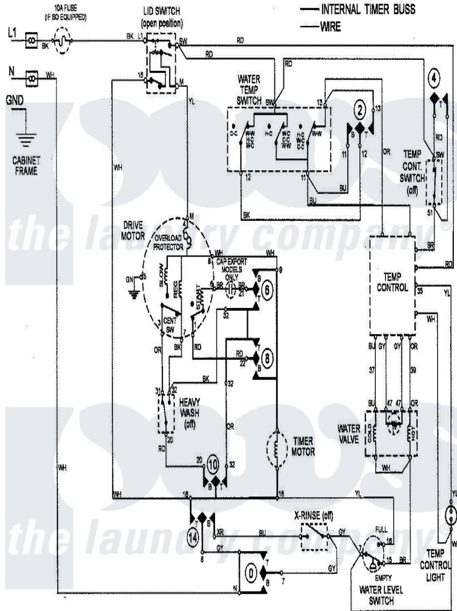
Maytag Residential Maytag MAV7357AWW Washer Parts Parts Diagram 08 - WIRING INFORMATION Click on the part number to view part
