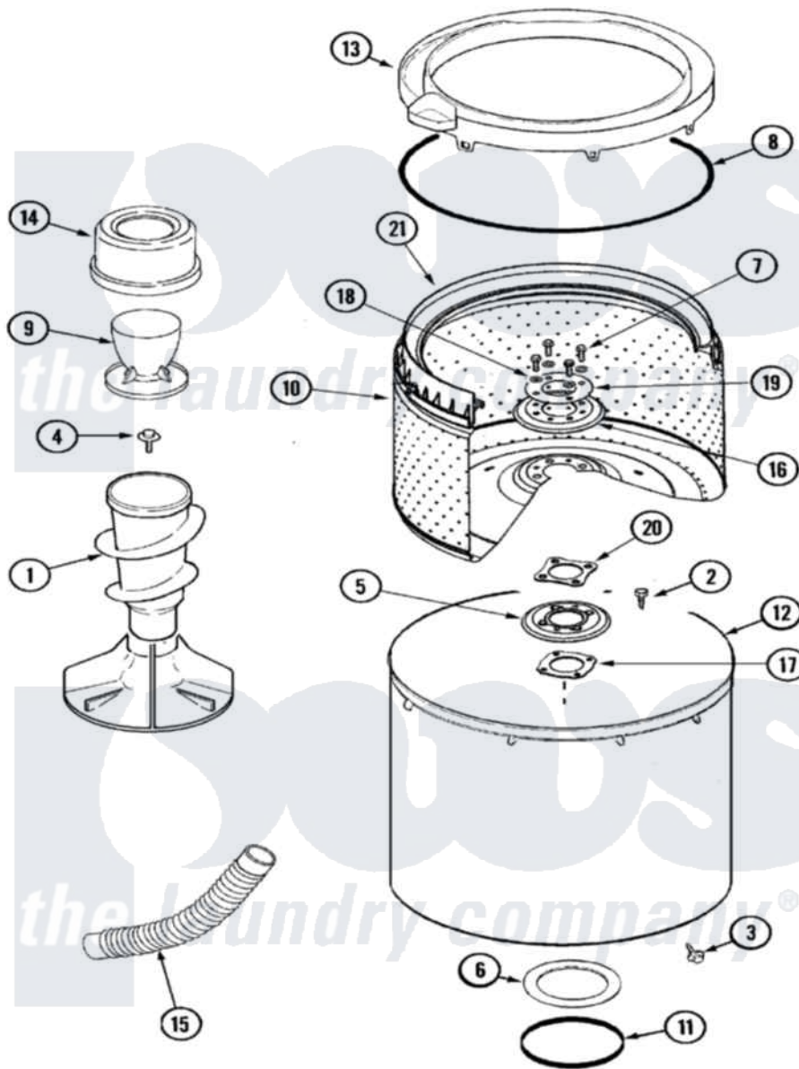
Maytag Residential Maytag MAV7550AWQ Washer Parts Parts Diagram 06 - TUB Click on the part number to view part
