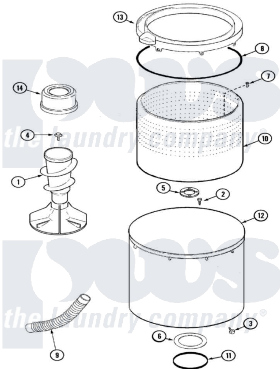
Maytag Residential Maytag MAV7557EWQ Washer Parts Parts Diagram 07 - TUB Click on the part number to view part
