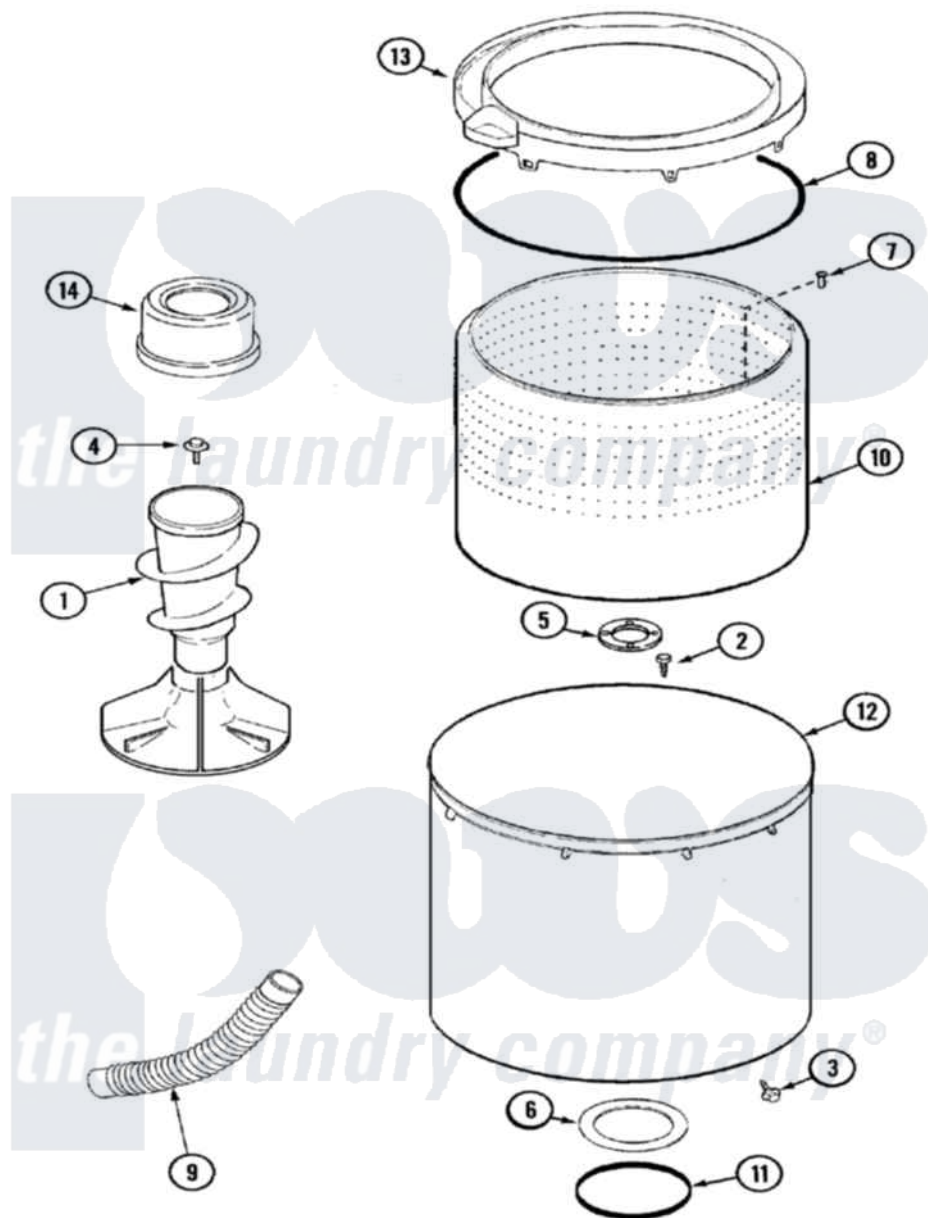
Maytag Residential Maytag MAV7557EWW Washer Parts Parts Diagram 07 - TUB Click on the part number to view part
