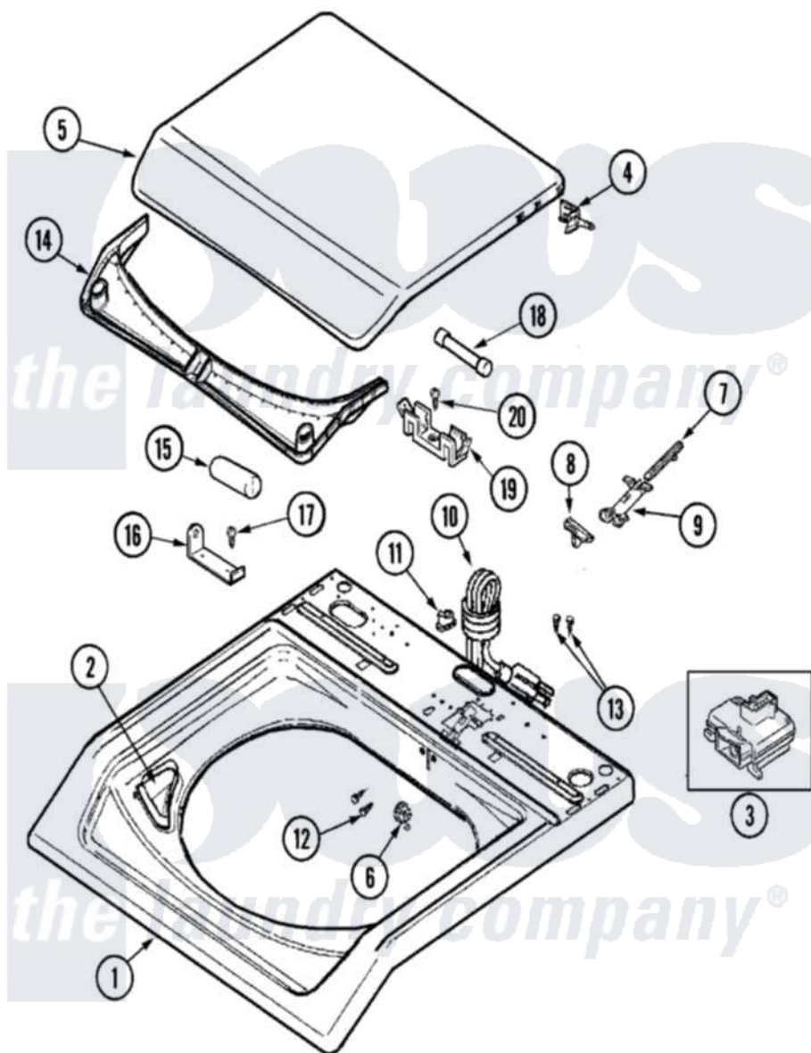
Maytag Residential Maytag MAV7600ACQ Washer Parts Parts Diagram 04 - TOP Click on the part number to view part
