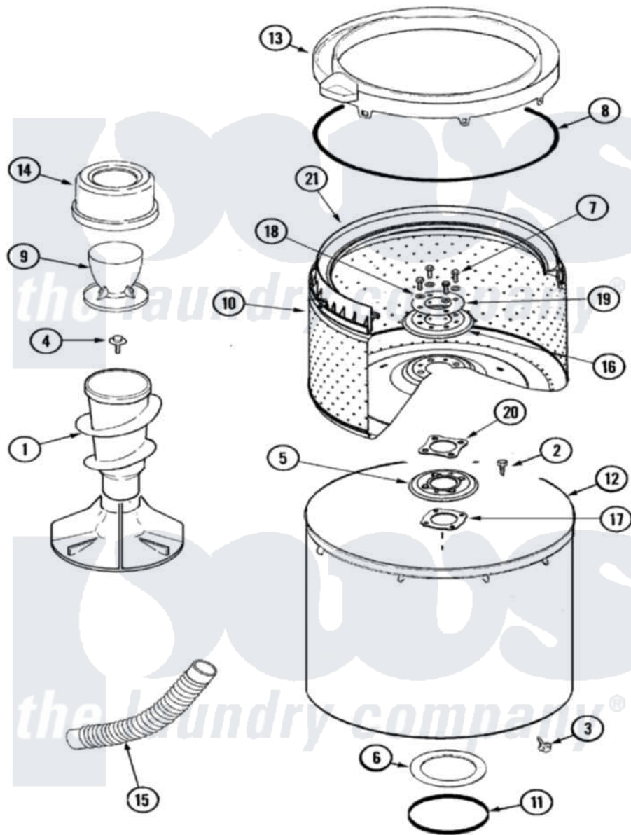
Maytag Residential Maytag MAV7700AWW Washer Parts Parts Diagram 07 - TUB Click on the part number to view part
