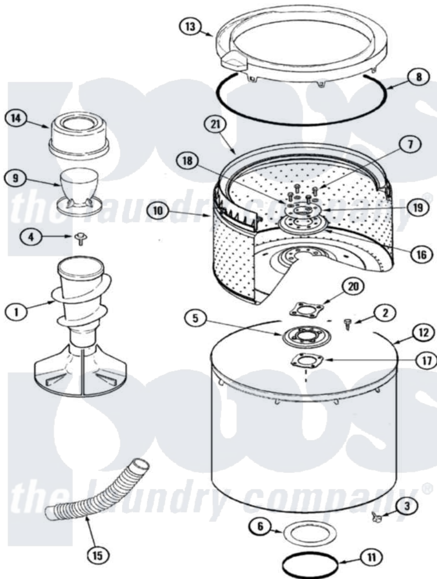
Maytag Residential Maytag MAV7757AWW Washer Parts Parts Diagram 07 - TUB Click on the part number to view part
