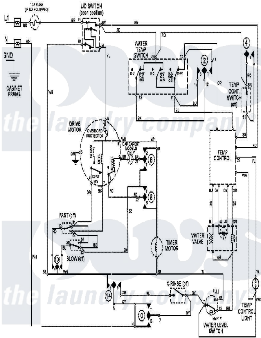
Maytag Residential Maytag MAV7757AWW Washer Parts Parts Diagram 08 - WIRING INFORMATION Click on the part number to view part
