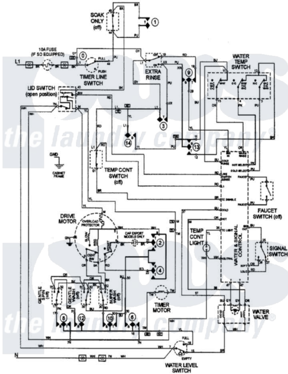
Maytag Residential Maytag MAV8057AWQ Washer Parts Parts Diagram 07 - WIRING INFORMATION Click on the part number to view part
