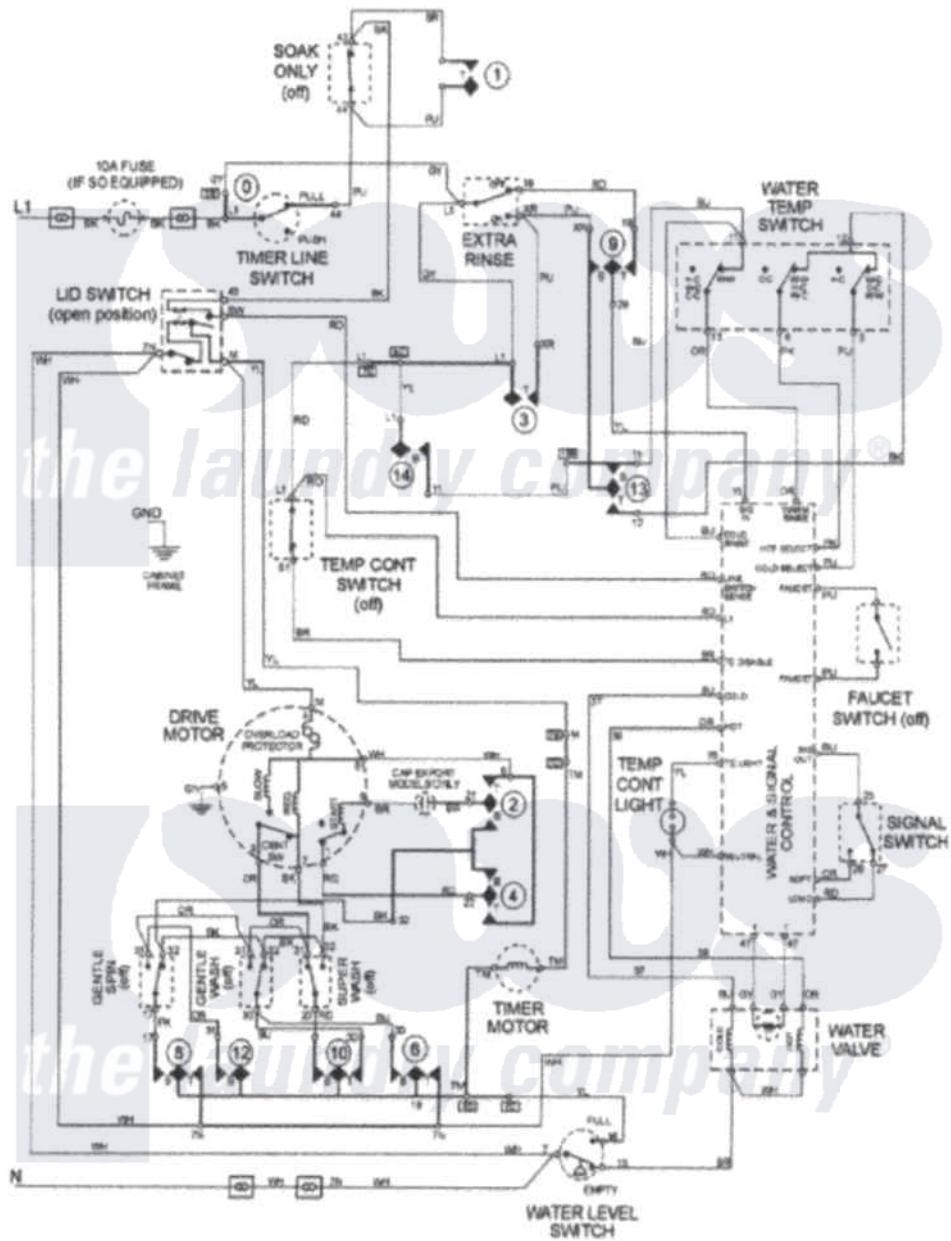
Maytag Residential Maytag MAV8057AWQ Washer Parts Parts Diagram 08 - WIRING INFORMATION Click on the part number to view part
