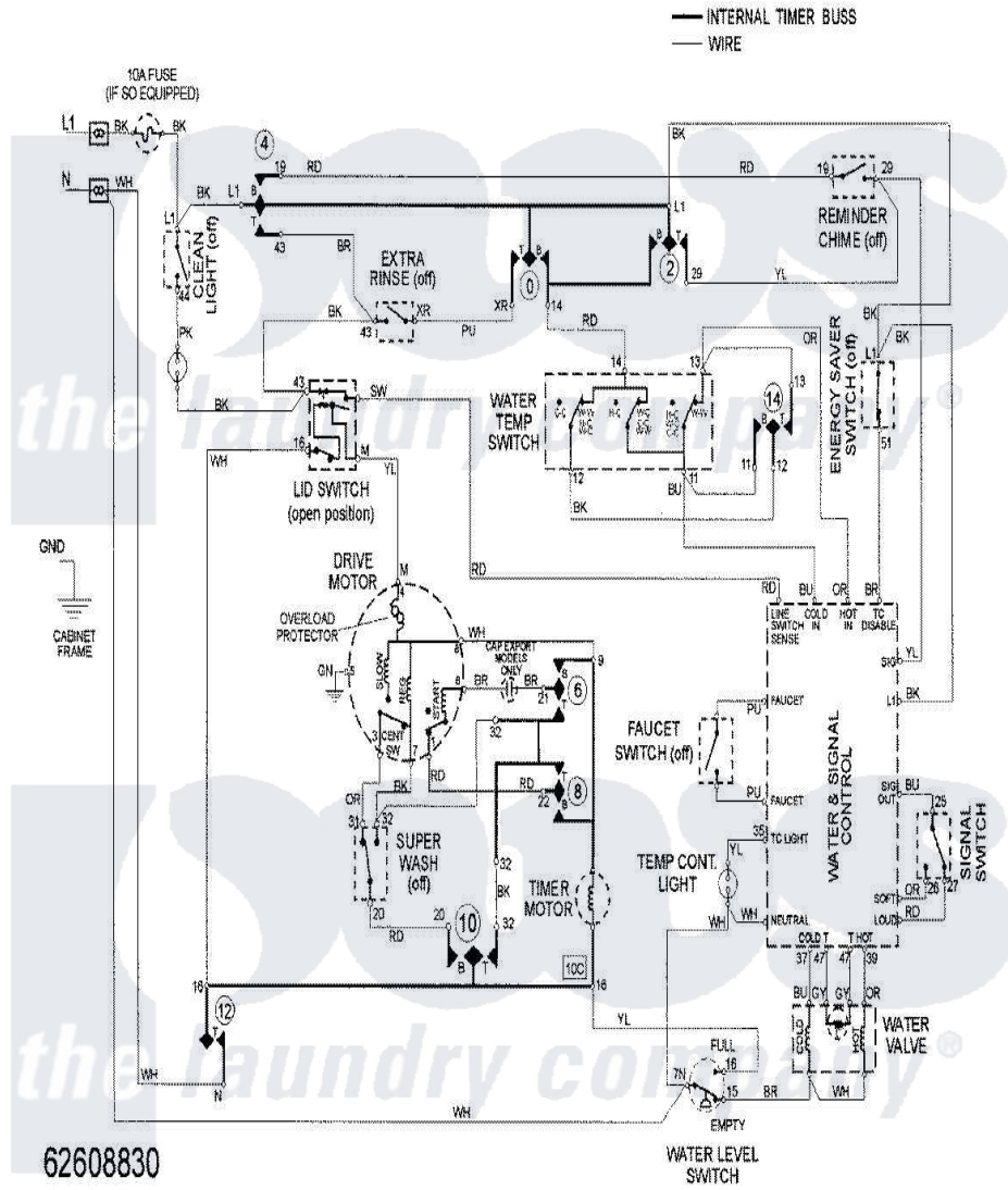
Maytag Residential Maytag MAV9600EWQ Washer Parts Parts Diagram 07 - WIRING INFORMATION Click on the part number to view part
