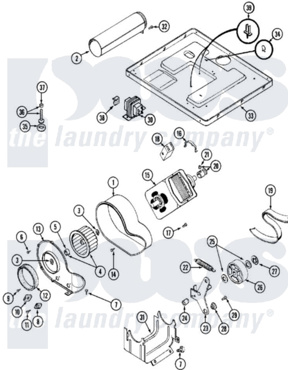
Maytag Residential Maytag MDE10PSAGL Dryer Parts Parts Diagram 08 - MOTOR DRIVE Click on the part number to view part
