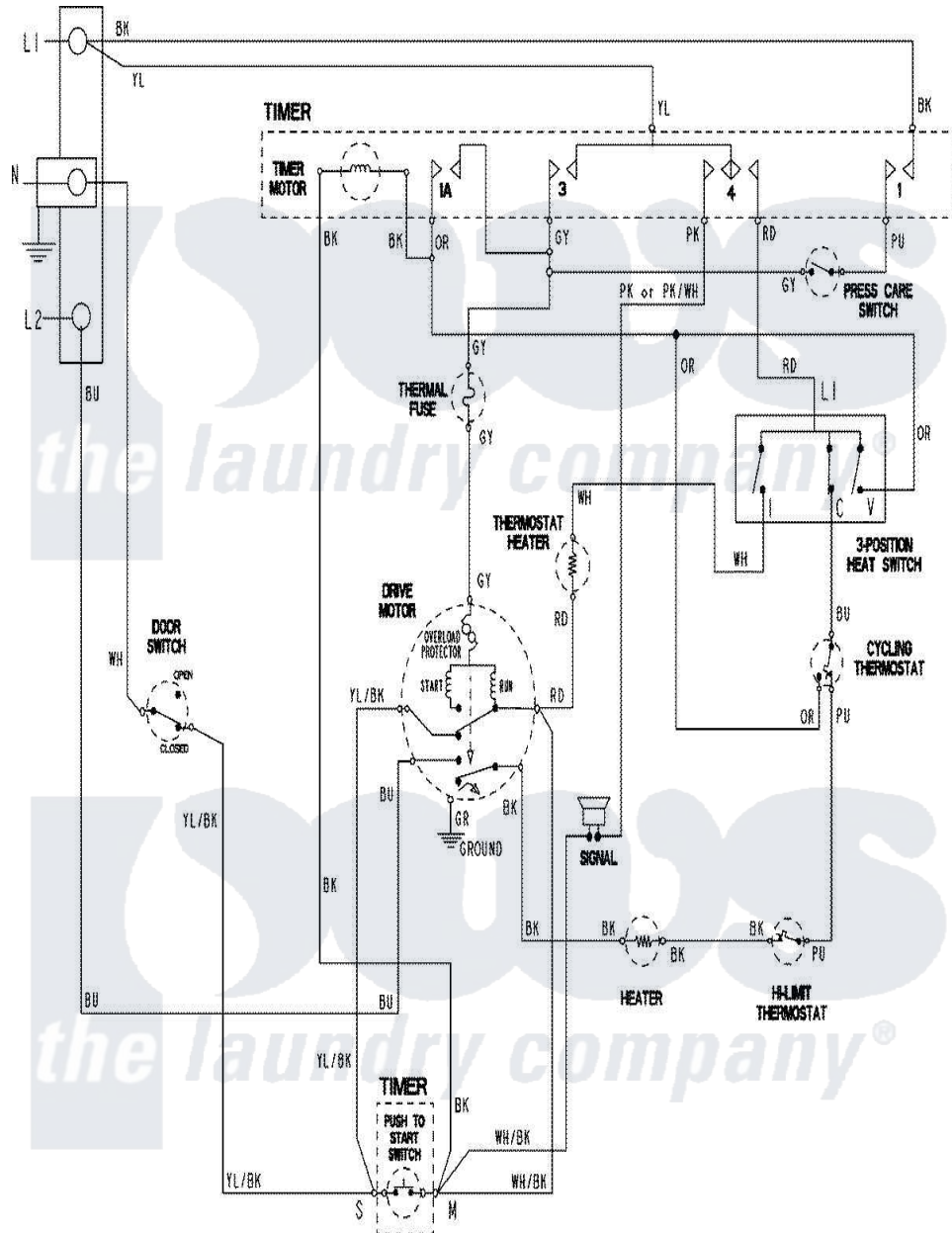
Maytag Residential Maytag MDE208DAYW Dryer Parts Parts Diagram 06 - WIRING INFORMATION Click on the part number to view part
