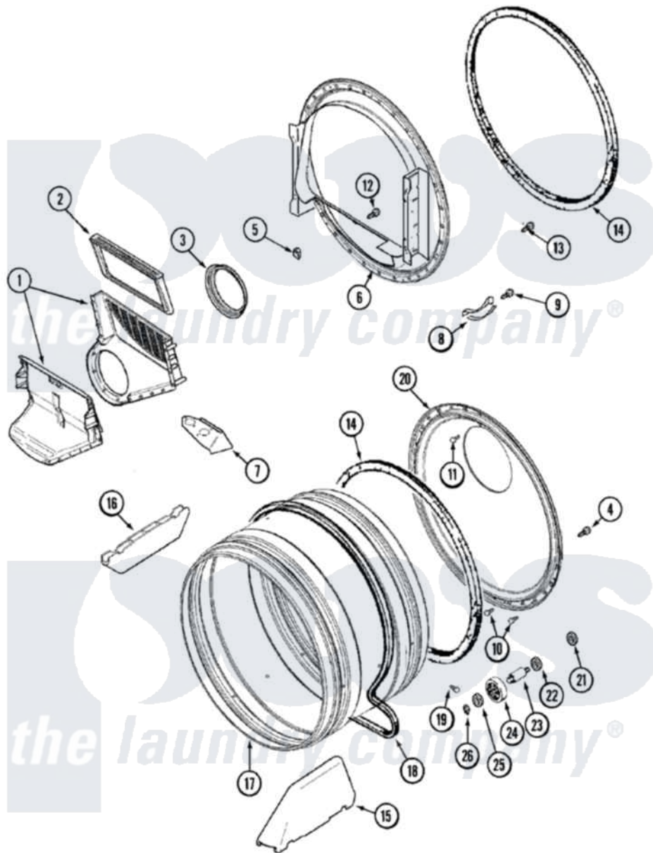
Maytag Residential Maytag MDE2600AZW Dryer Parts Parts Diagram 06 - TUMBLER Click on the part number to view part
