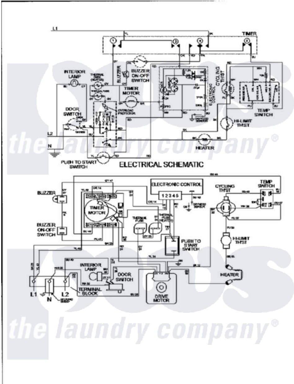
Maytag Residential Maytag MDE3600AYQ Dryer Parts Parts Diagram 09 - WIRING INFORMATION Click on the part number to view part
