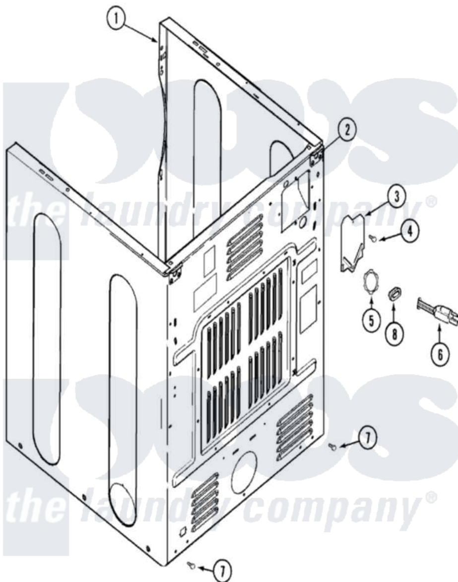
Maytag Residential Maytag MDE4916AYA Dryer Parts Parts Diagram 02 - CABINET-REAR Click on the part number to view part
