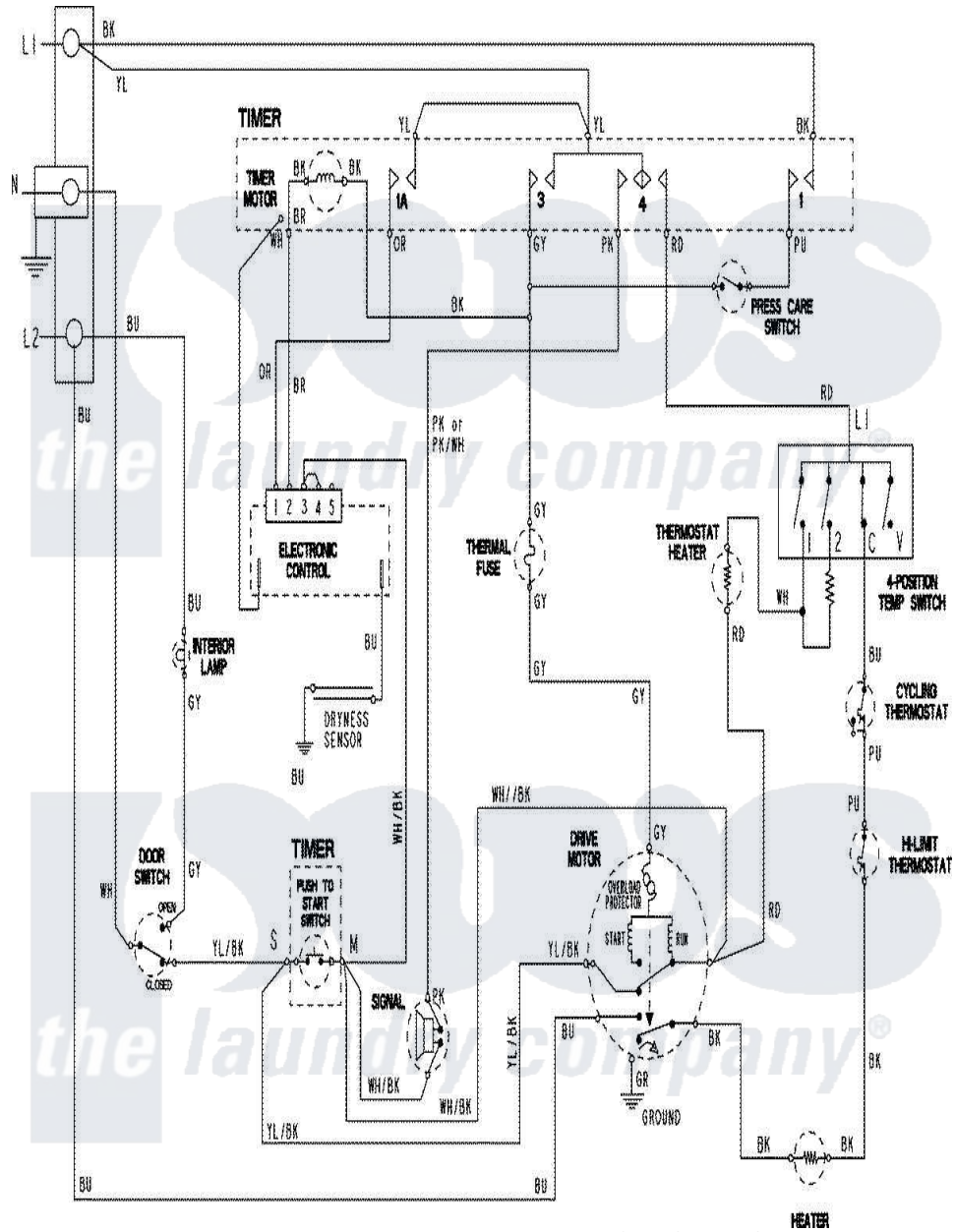
Maytag Residential Maytag MDE508DAYW Dryer Parts Parts Diagram 07 - WIRING INFORMATION Click on the part number to view part
