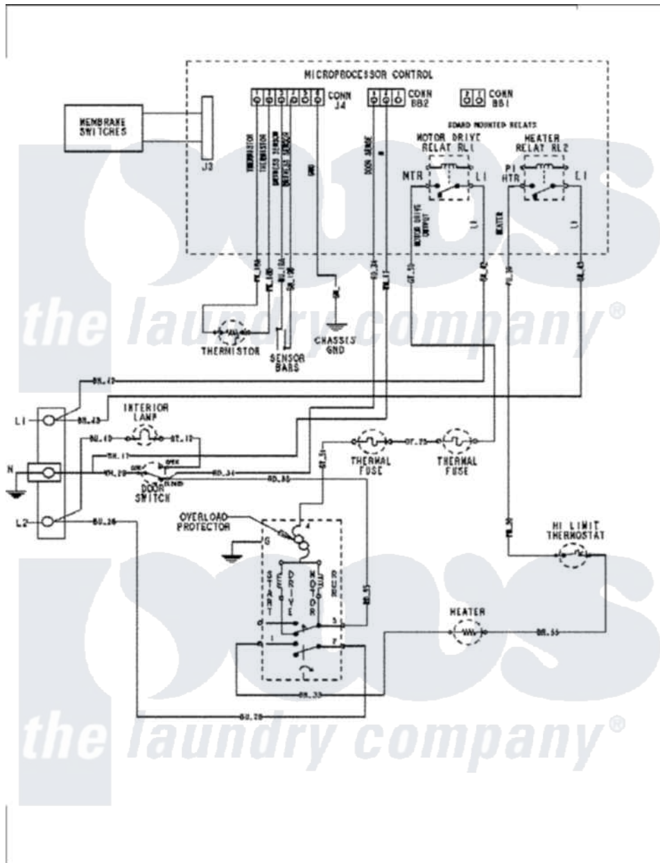
Maytag Residential Maytag MDE5500AYQ Dryer Parts Parts Diagram 09 - WIRING INFORMATION SERIES 62 AND LATER
