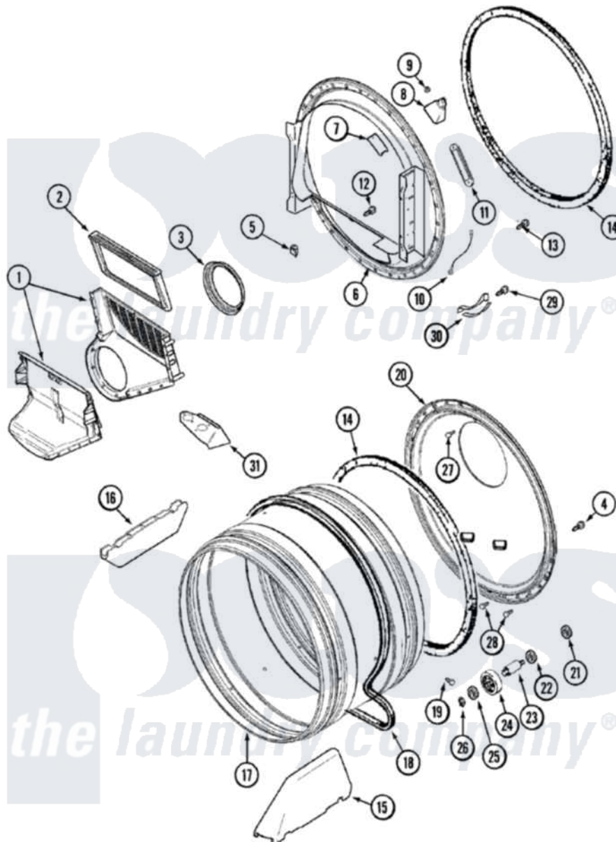
Maytag Residential Maytag MDE5500AZQ Dryer Parts Parts Diagram 05 - TUMBLER Click on the part number to view part
